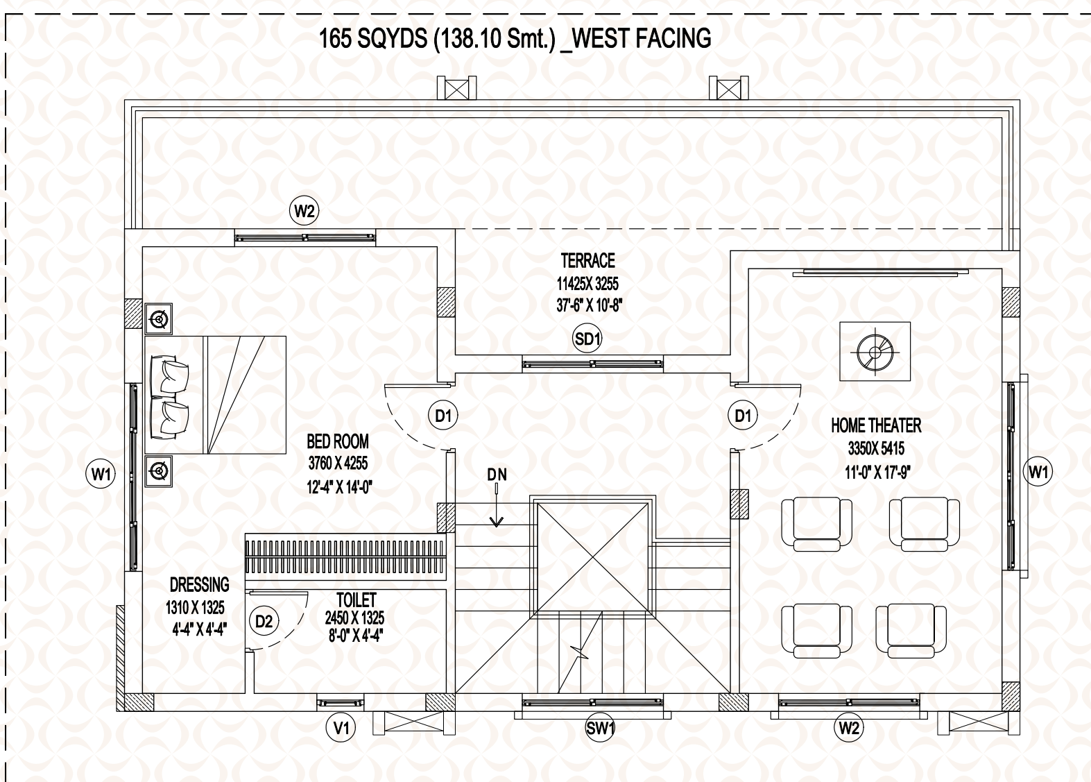
1 SECOND FLOOR PLAN
