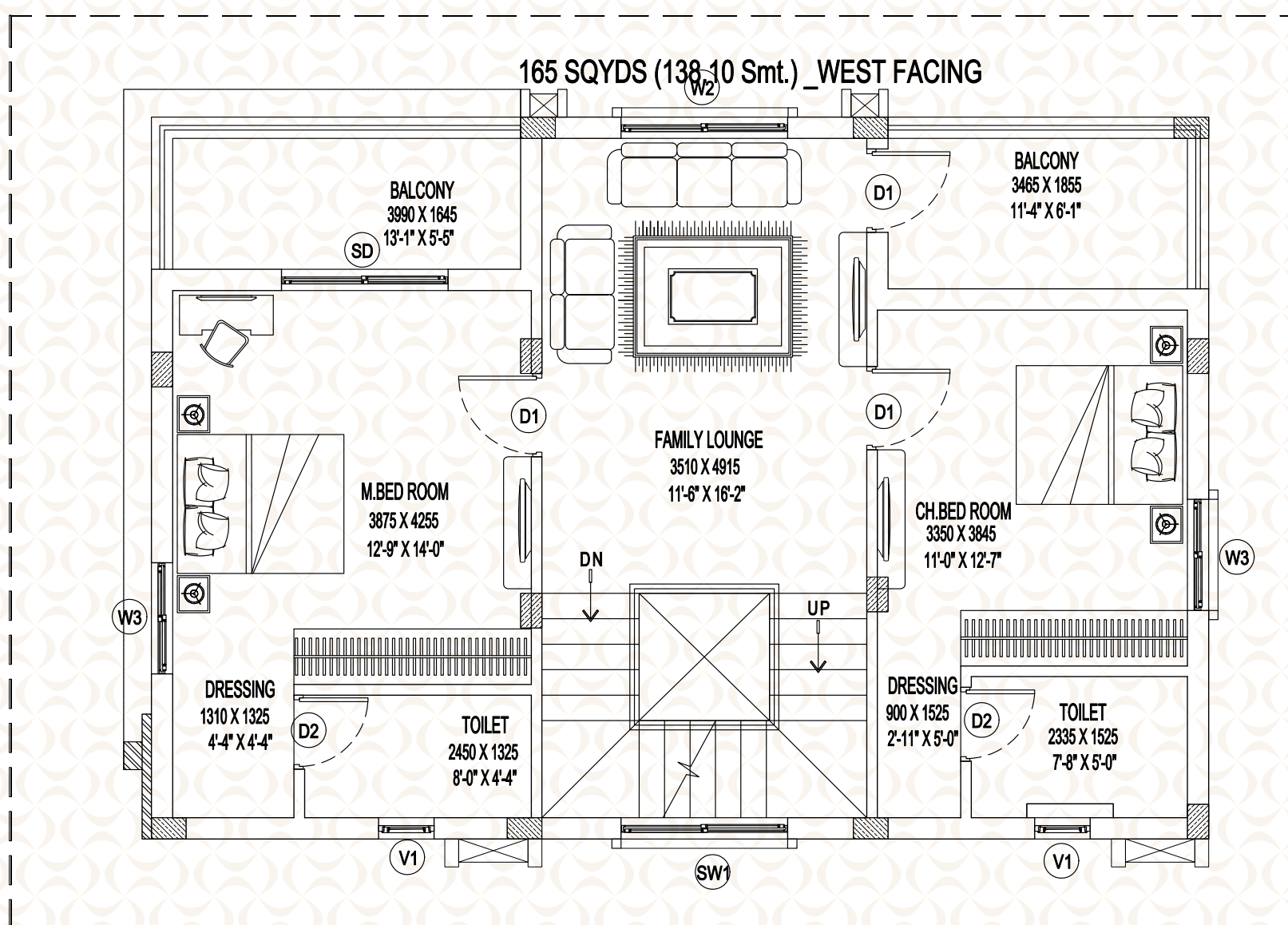
1 FIRST FLOOR PLAN
