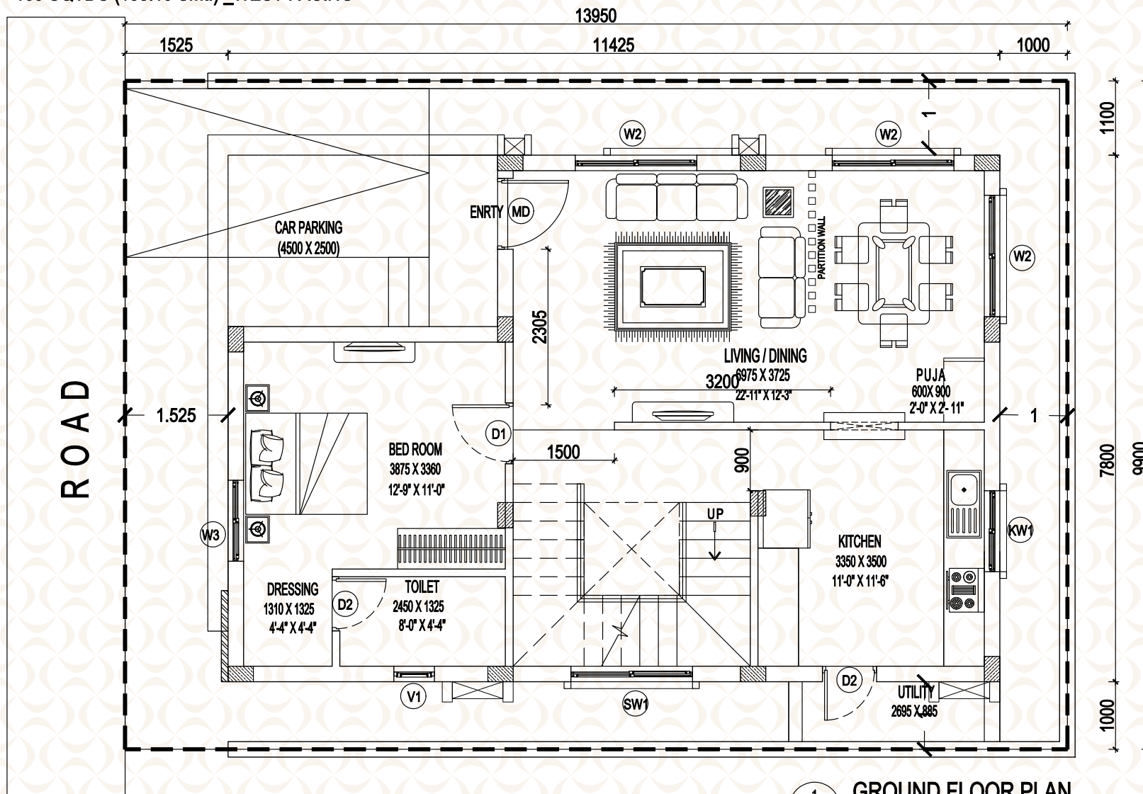
1 GROUND FLOOR PLAN
