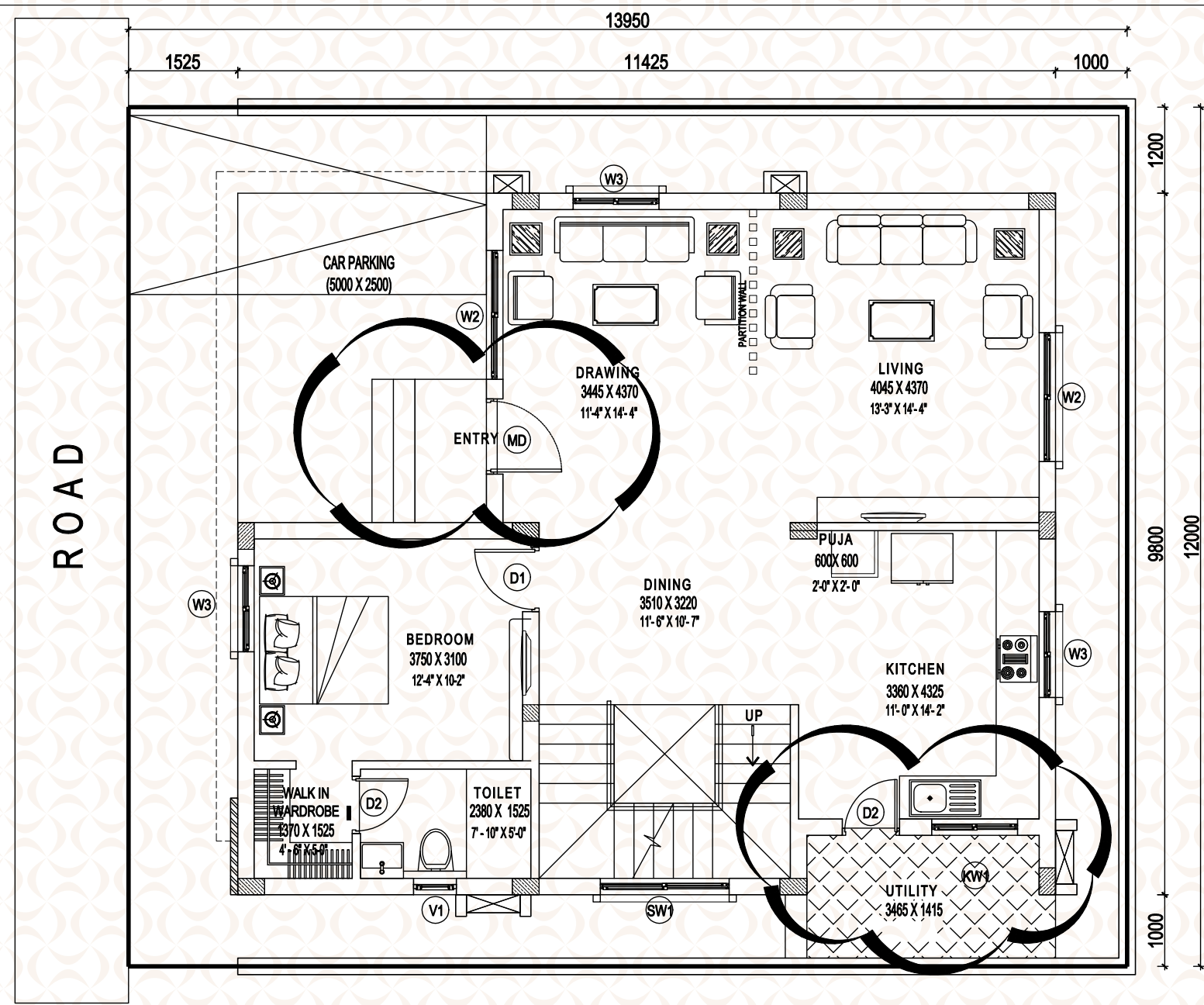
1 GROUND FLOOR PLAN
