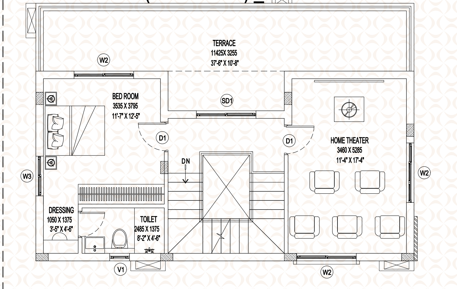
1 SECOND FLOOR PLAN
