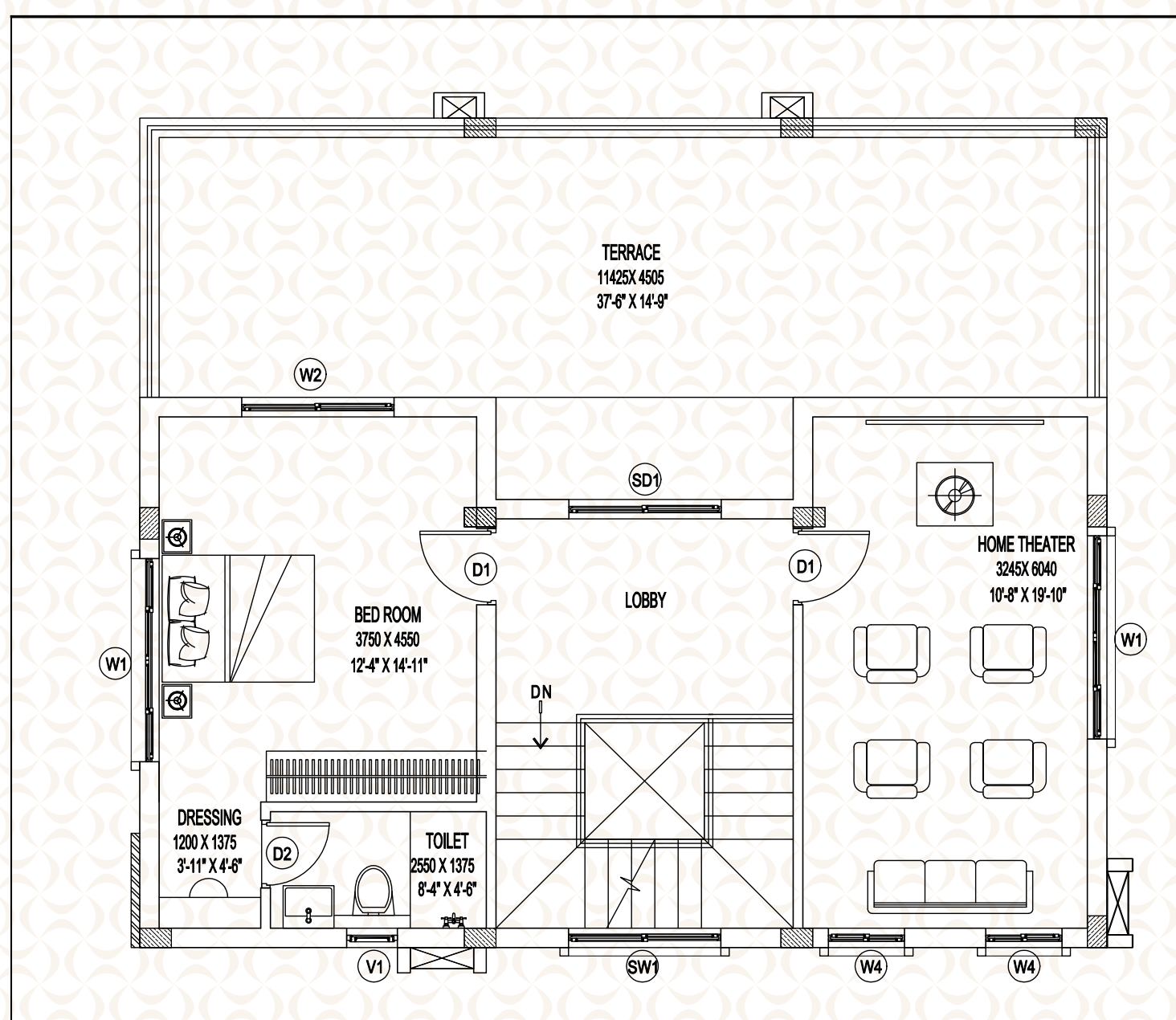
3 SECOND FLOOR PLAN
