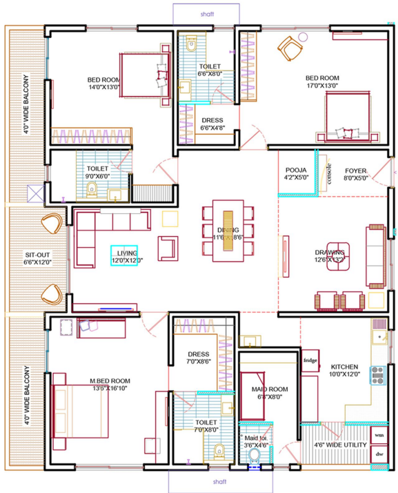
SIZE: 2880 SFT EAST FACING 3 BHK
