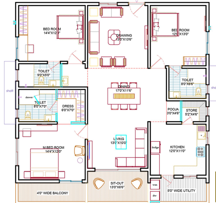
SIZE: 2315 SFT NORTH FACING 3 BHK
