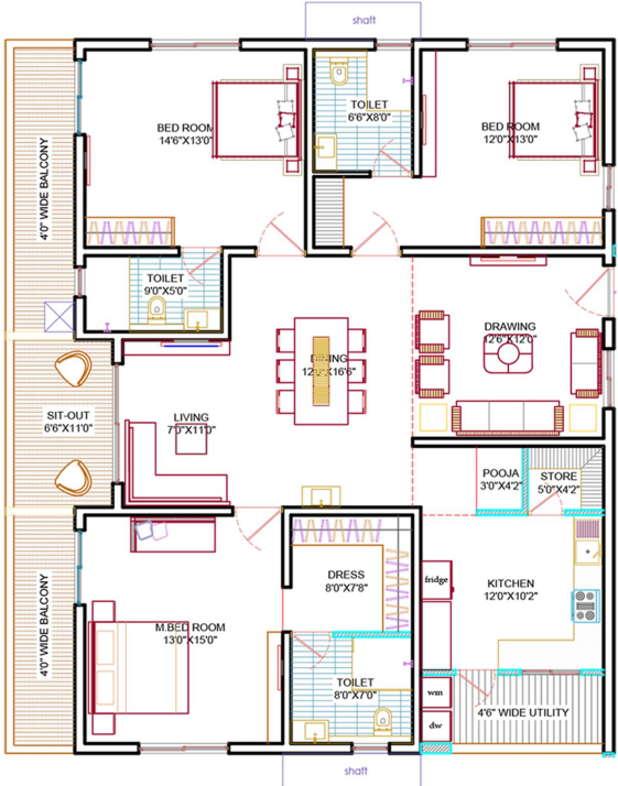
SIZE: 2390 SFT EAST FACING 3 BHK
