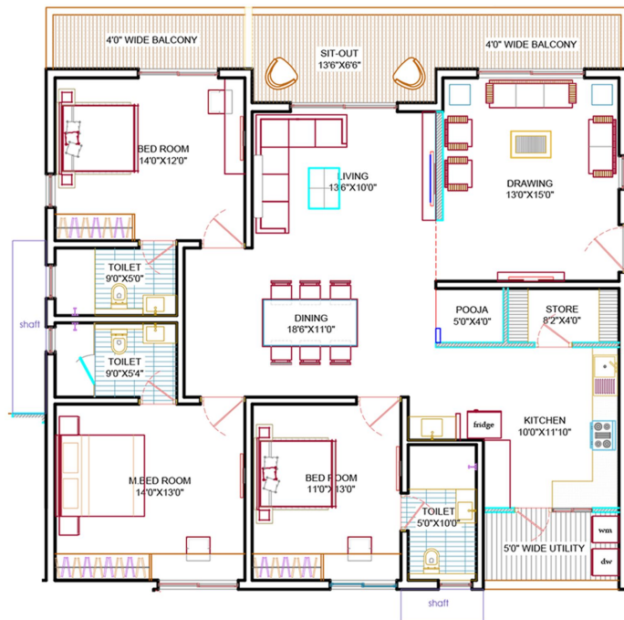
SIZE: 2355 SFT EAST FACING 3 BHK
