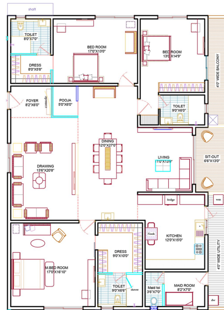
SIZE: 2675 SFT EAST FACING 3 BHK
