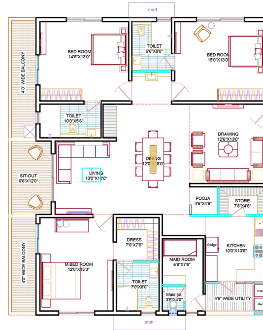
SIZE: 2675 SFT EAST FACING 3 BHK
