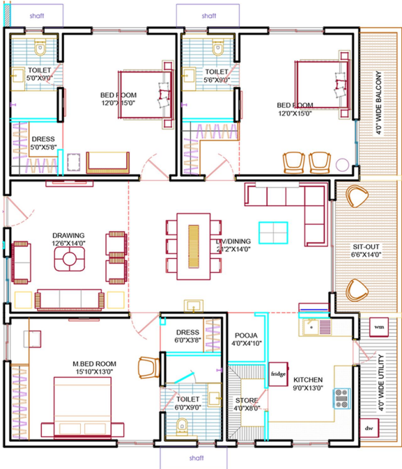
SIZE: 2390 SFT WEST FACING 3 BHK
