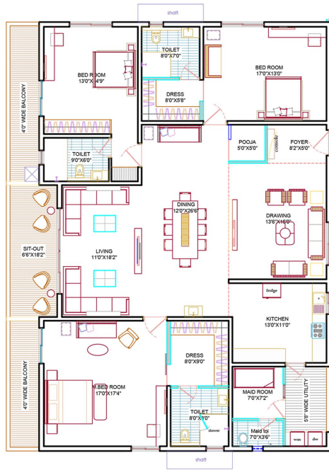
SIZE: 3400 SFT EAST FACING 3 BHK
