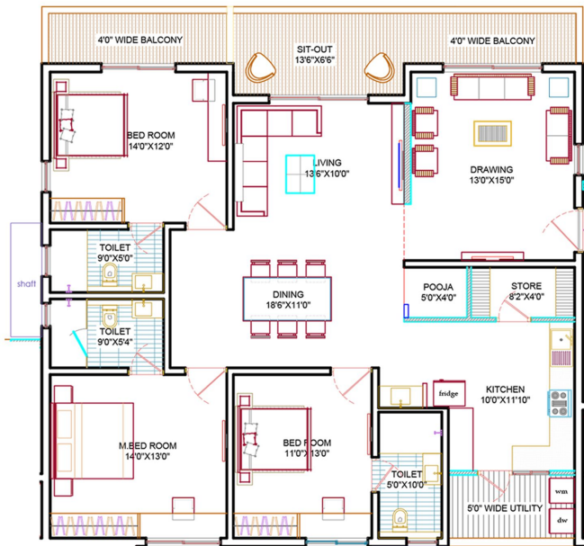
SIZE: 2355 SFT EAST FACING 3 BHK
