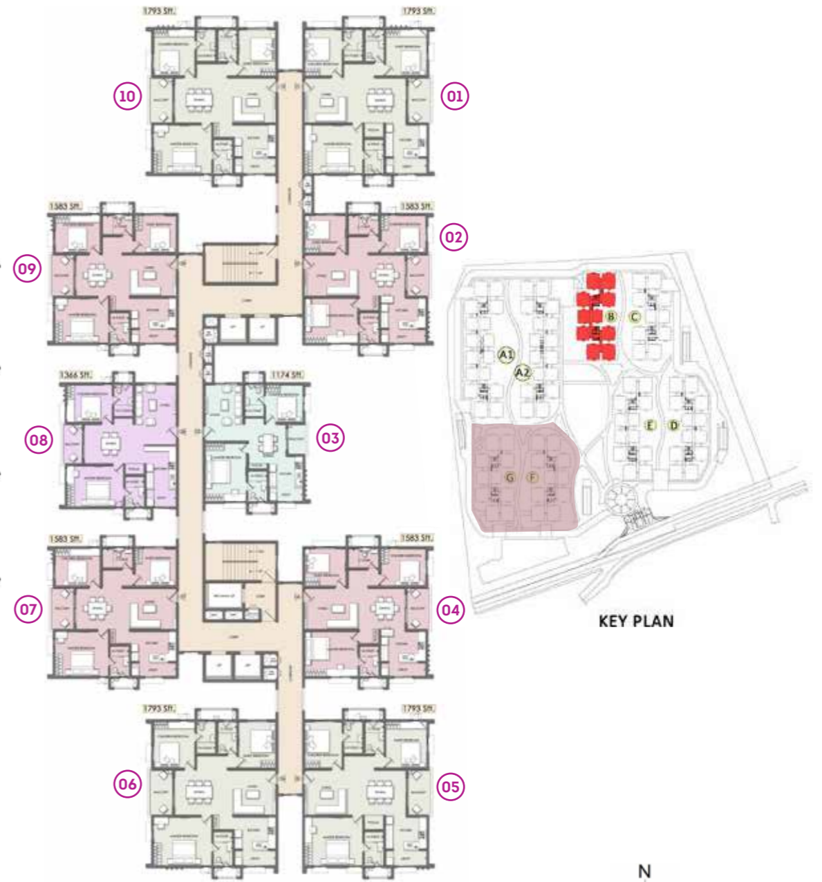
BLOCK-B 2nd TO 15th FLOOR PLAN (TYPICAL FLOOR PLAN)
