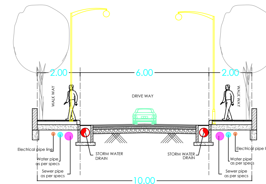
SECTION (10 M WIDE ROAD)
