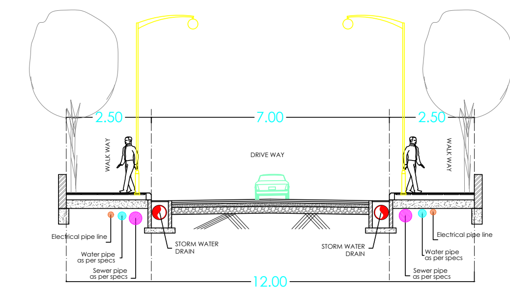
SECTION (12 M WIDE ROAD)
