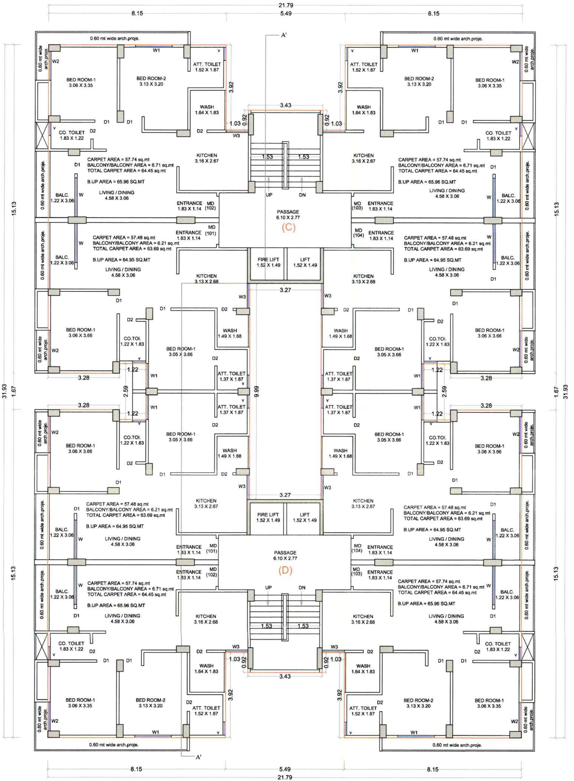
TYPICAL FLOOR PLAN(1st TO 7th) SCALE :- 1CM=1MT.
