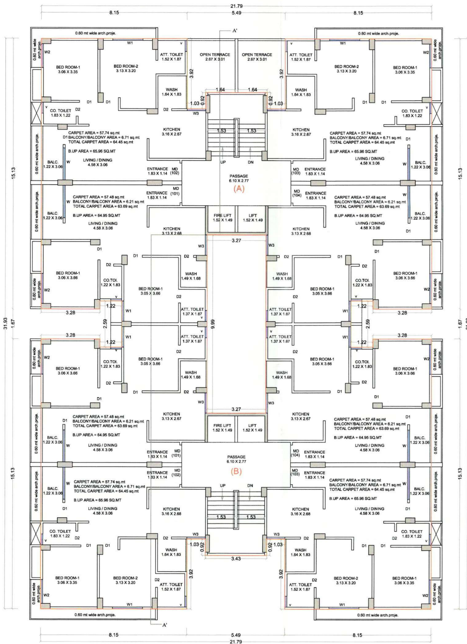
FIRST FLOOR PLAN SCALE :- 1CM=1MT.
