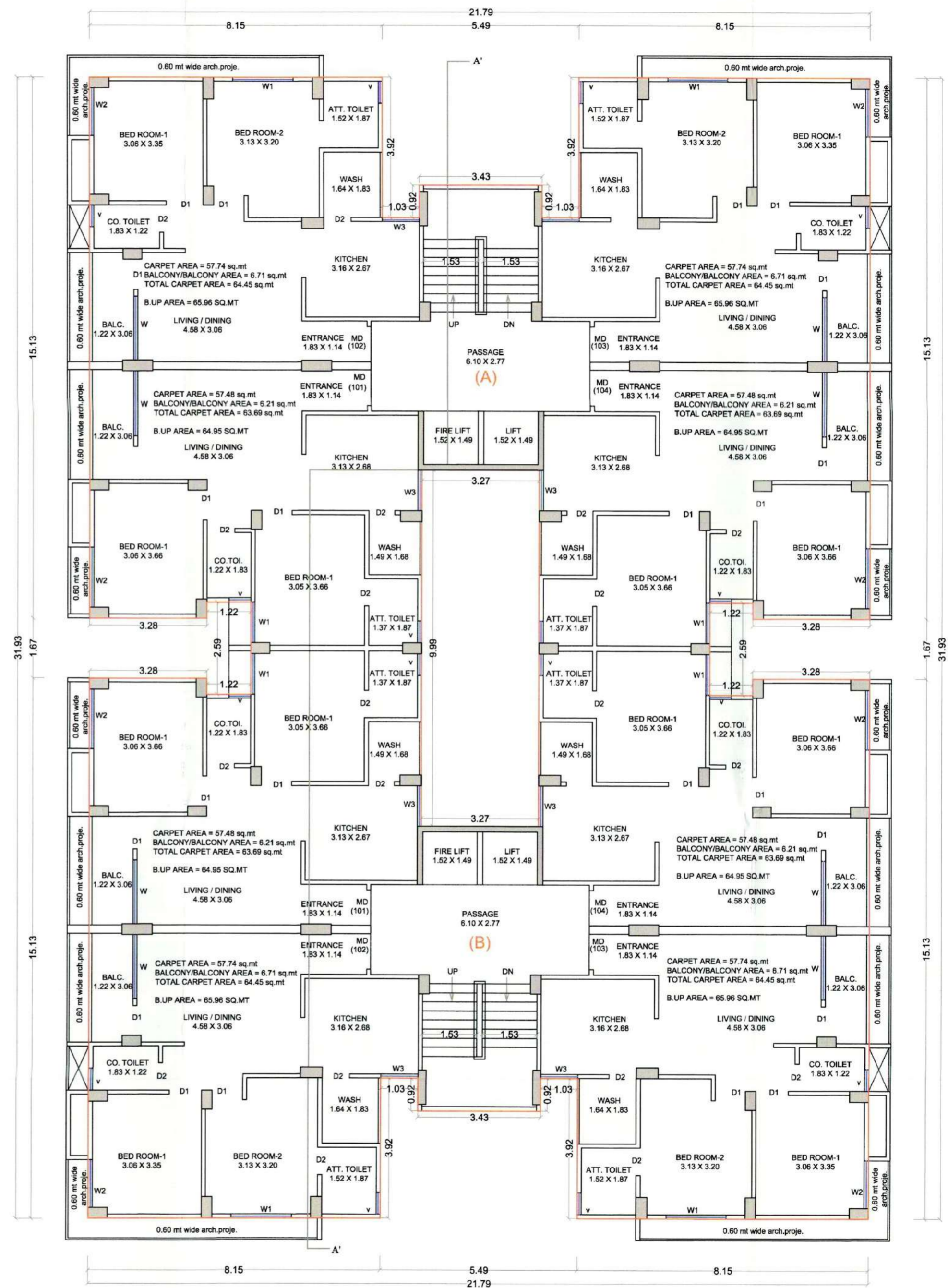
TYPICAL FLOOR PLAN (2nd TO 6th) SCALE :- 1CM=1MT.
