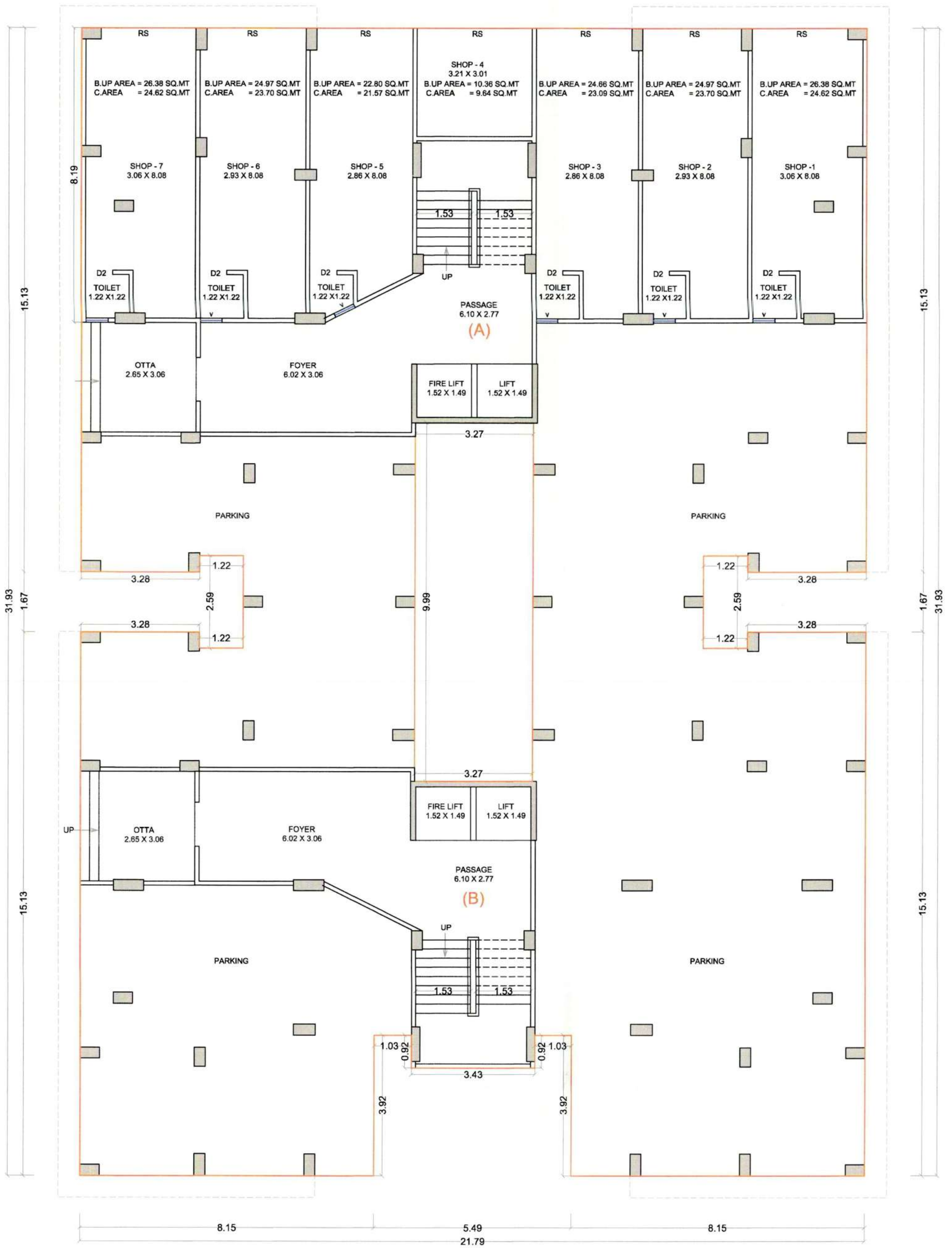
GROUND FLOOR PLAN SCALE :- 1CM=1MT.
