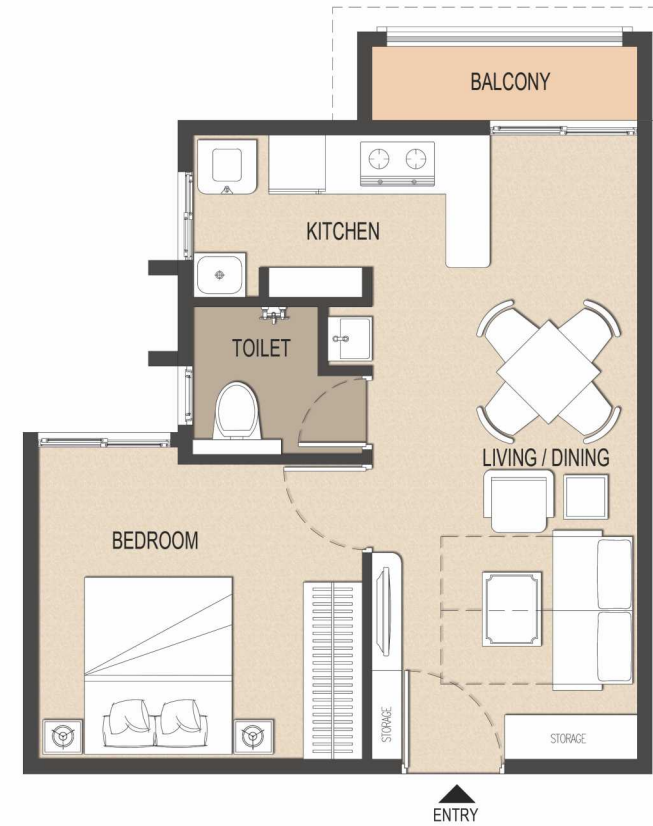
1 BHK TYPICAL FLOOR PLAN TYPE B
