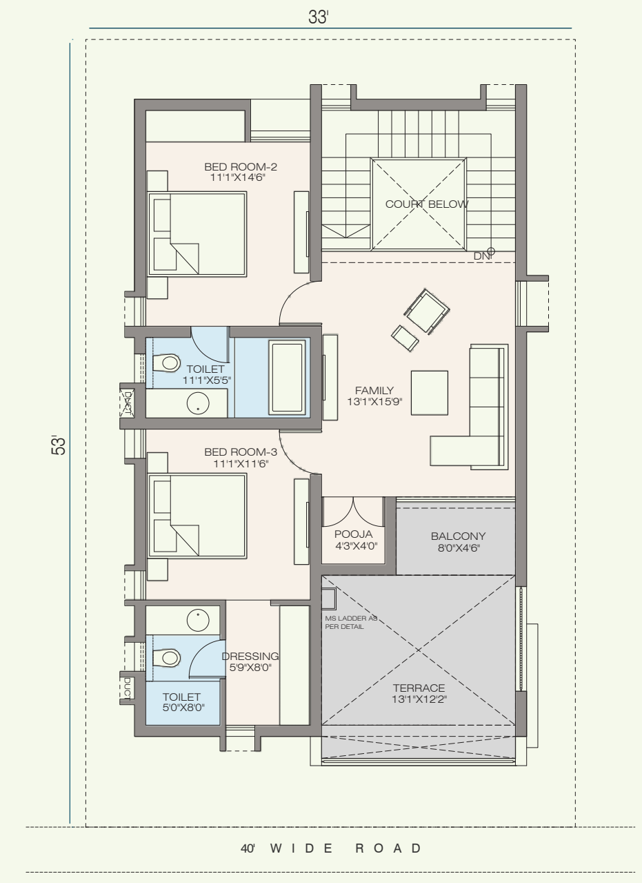
FIRST FLOOR: 983 SFT
