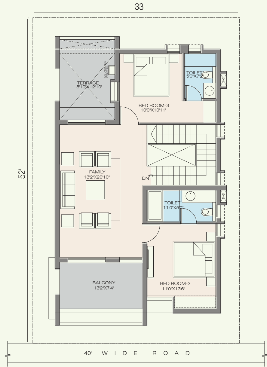
FIRST FLOOR: 1035 SFT
