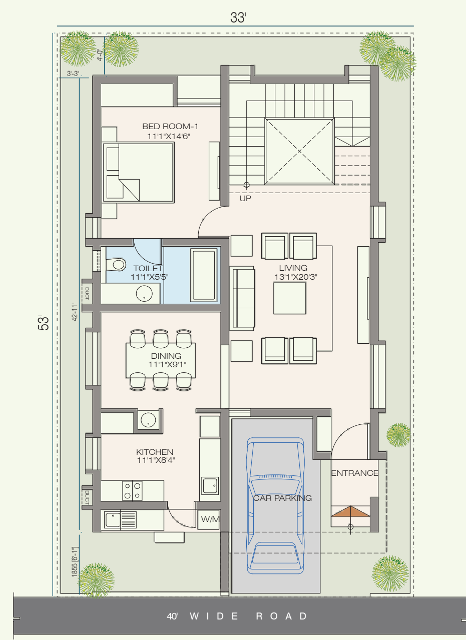
GROUND FLOOR: 1161 SFT
