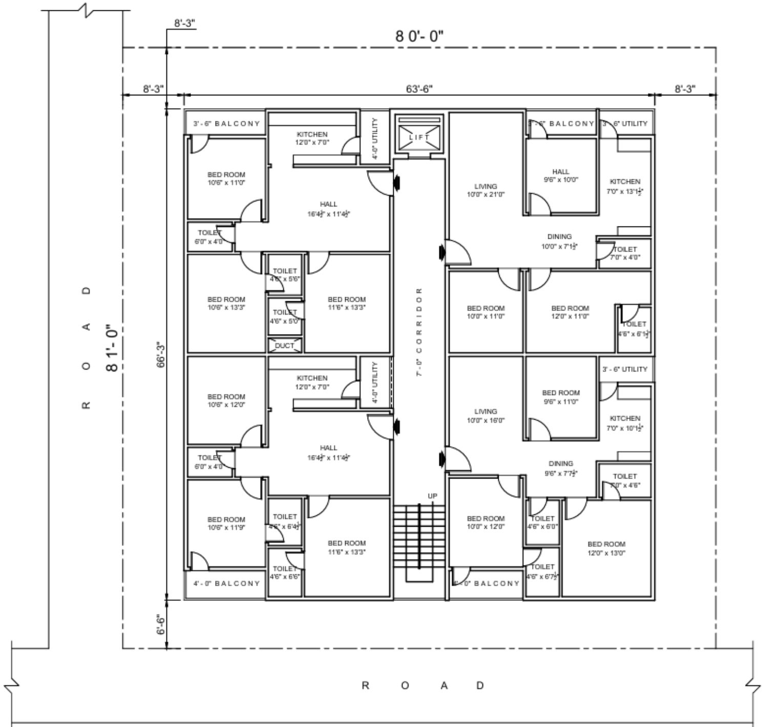
THIRD & FOURTH FLOOR PLAN - OPTION - 7 - (20-07-2023)
